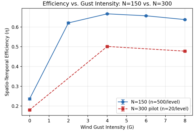
Fig. 4: Efficiency vs. gust intensity at N = 150 (full study, n = 500 per level) and N = 300 (preliminary comparison, n = 20 per level). The qualitative pattern – zero-gust collapse, peak at moderate gust – holds at both population sizes, though absolute efficiency is systematically lower at N = 300 .
